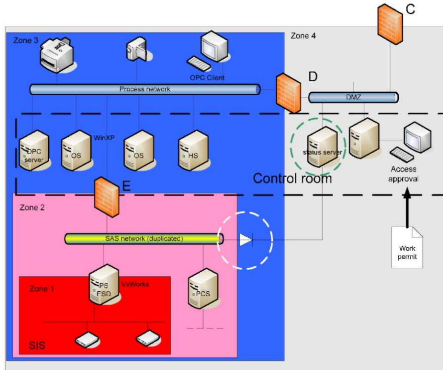
Figure 5 Introduction of information diode for read-only access (see online version for colours)
