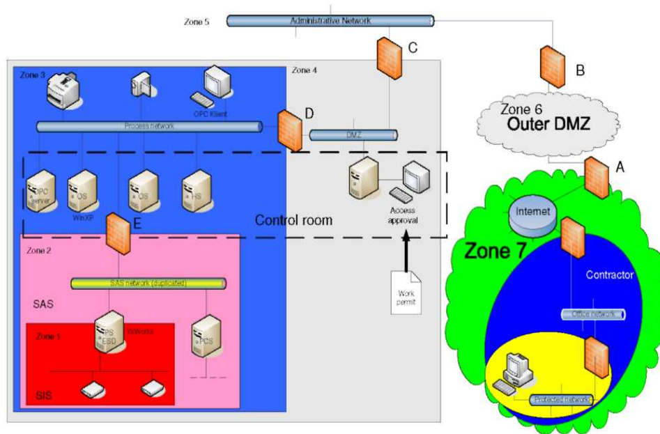
Figure 4 Case for remote access (see online version for colours)
